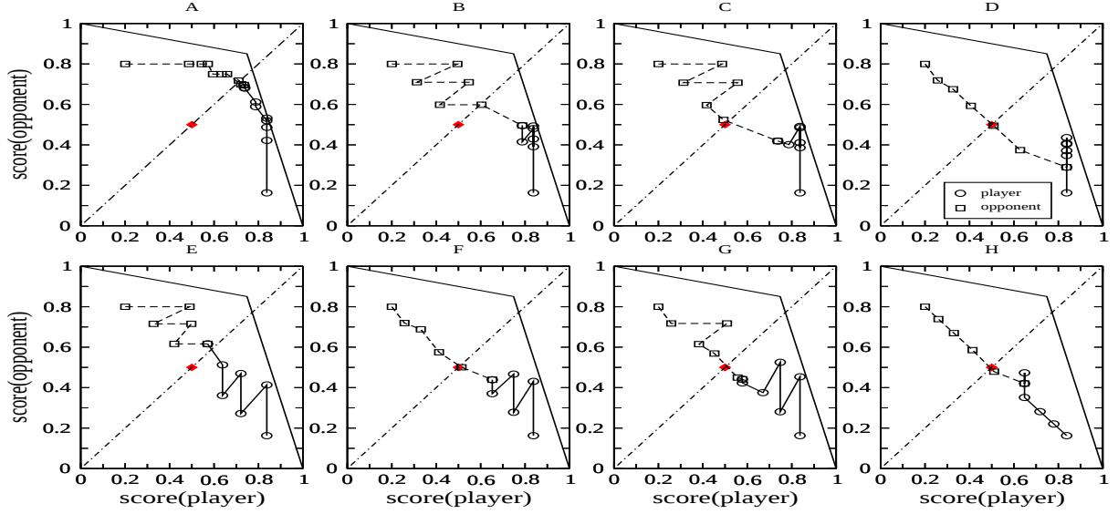
Figure 7: Dynamics of negotiation process for meta strategies: A) smart v. smart, B) smart v. serial, C) smart v. random D) smart v. responsive, E) serial v. serial, F) serial v. responsive, G) random v. random, H) random v. responsive.
