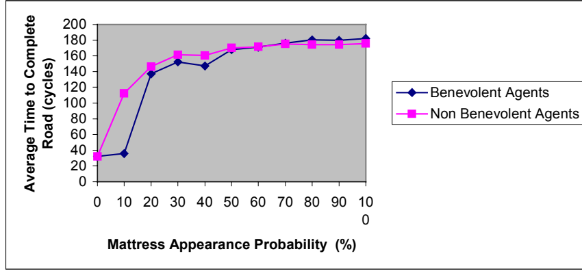
Figure 6: Average completion time vs. Mattress appearance probability
